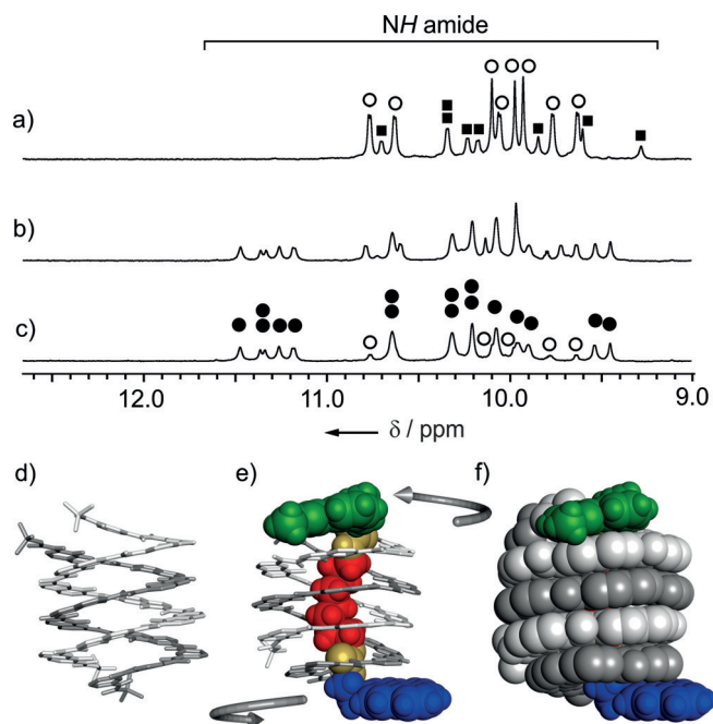
Figure 3. Partial ^1\text{H} NMR spectra (300 MHz, 298 K) showing the amide region of ( 4 ) 2 (2 mM) in \text{CDCl}_3 : a) in the absence of guest, b), c) in the presence of 1 b) 0.5 equiv and c) 2 equiv guest. The signals of the empty parallel and antiparallel double helix ( 4 ) 2 are marked with \circ and \square , respectively. The signals of 1C(4) 2 are denoted with \bullet . d)–f) Solid-state structures [16] of d) the free antiparallel double helix ( 4 ) 2 , e), f) the foldaxane 2C(4) 2 . The antiparallel strands of ( 4 ) 2 are shown in gray and white tube (d,e) and CPK (f) representations. The rod-like guest 2 is shown in CPK representation. The bipyridine and the pyrene stoppers are shown in green and blue, respectively. The carbamate functions and the linear alkyl chain of the guest are shown in gold and red, respectively. The gray arrows illustrate the unscrewing motion of ( 4 ) 2 to accommodate the guest. [7d]
