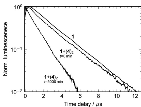
Figure 4. Luminescence decays on the microsecond timescale of free thread 1 (50 \mu\text{M} ) and host-guest mixture (32:1, 2 mM of host) immediately after mixing ( t=0 min) and at t=5000 min, when 77.5% formation of complex 1C(4) 2 is attained ( \lambda_{\text{ex}}=465 nm, \lambda_{\text{obs}}=620 nm) in \text{CDCl}_3 .
